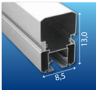
ΟΔΗΓΟΣ PERGO IDEAL 130
